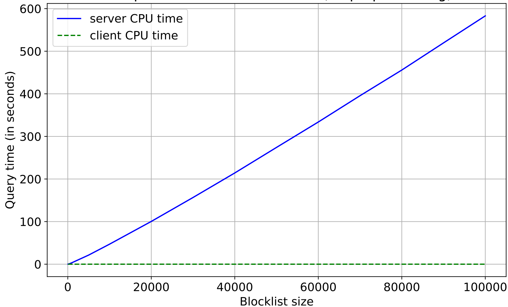
Compute time vs. Blocklist size (no preprocessing)
